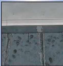
Before - Open seams and deteriorated surface on modified bitumen membrane on sloped wall
